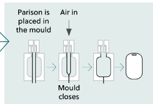
Blow moulding of liner
